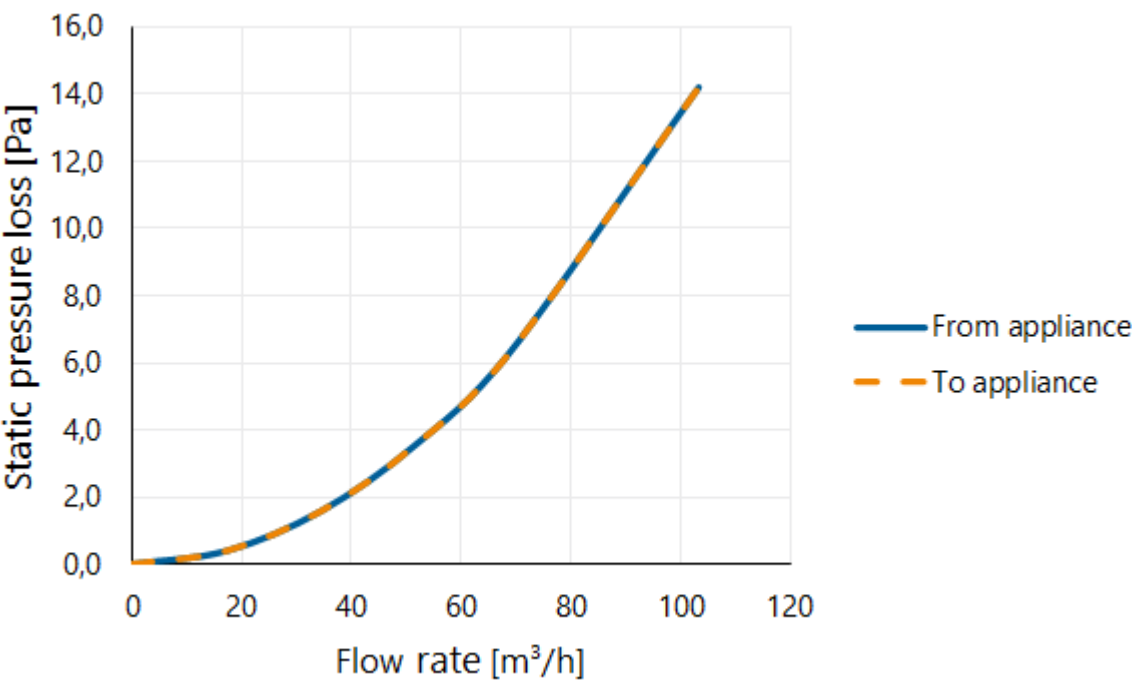
Pressure loss
