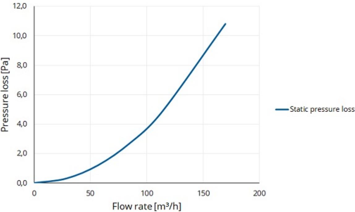
Pressure loss per meter versus flow rate
