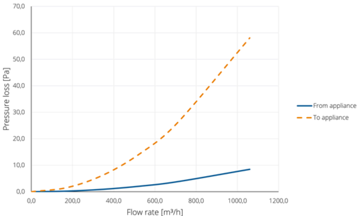
Pressure loss
