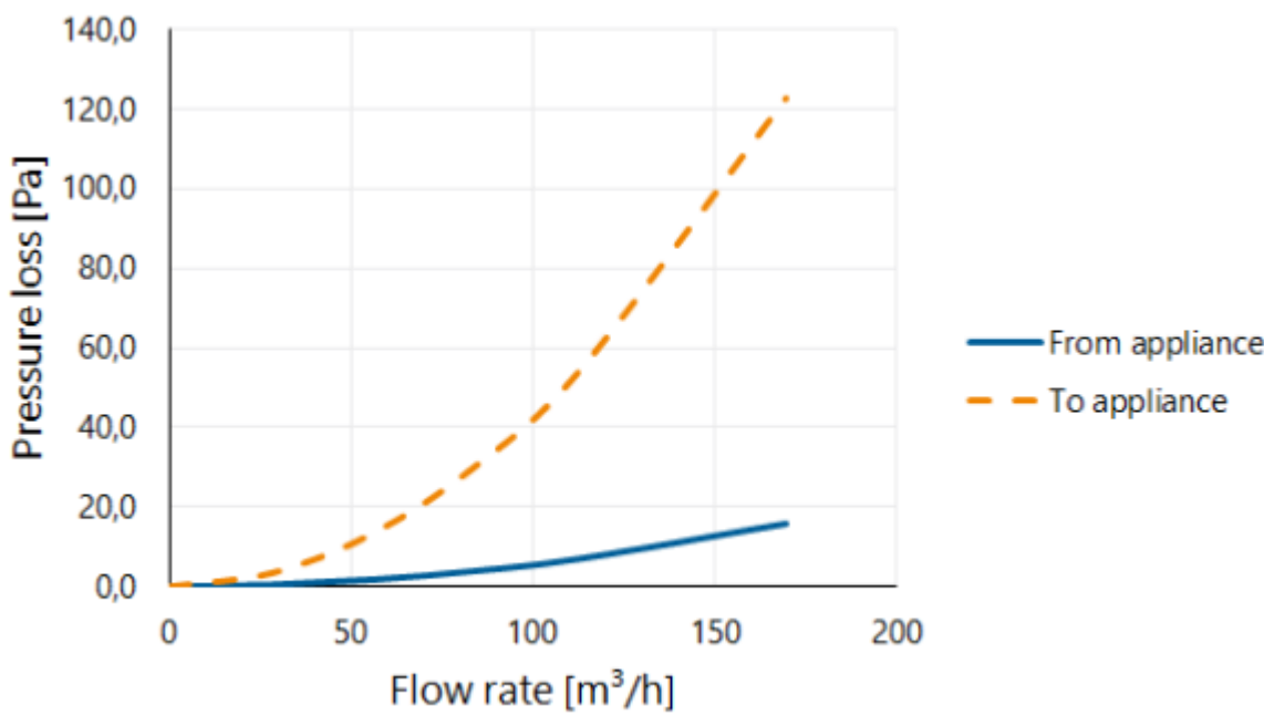
Pressure loss
